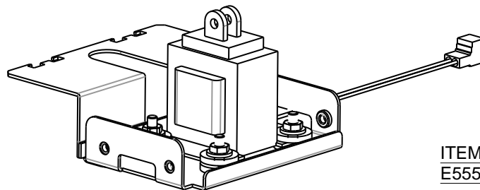
ITEM 36 - SOLENOID SHELF ASSY
